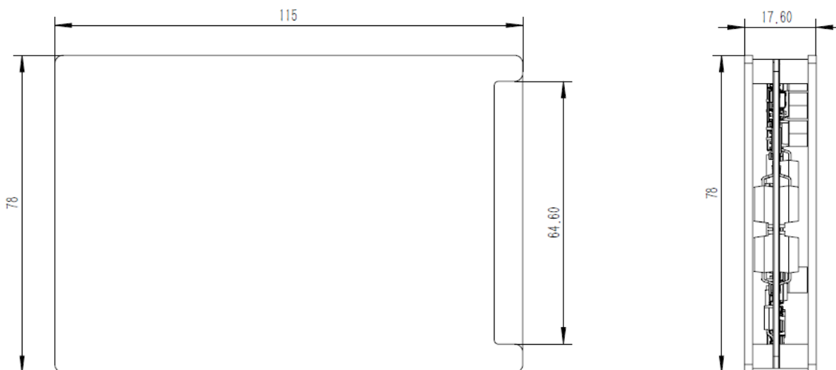
Figure 6. Outline Dimension Drawing of BD6A17S6P/BD6A20S6P
