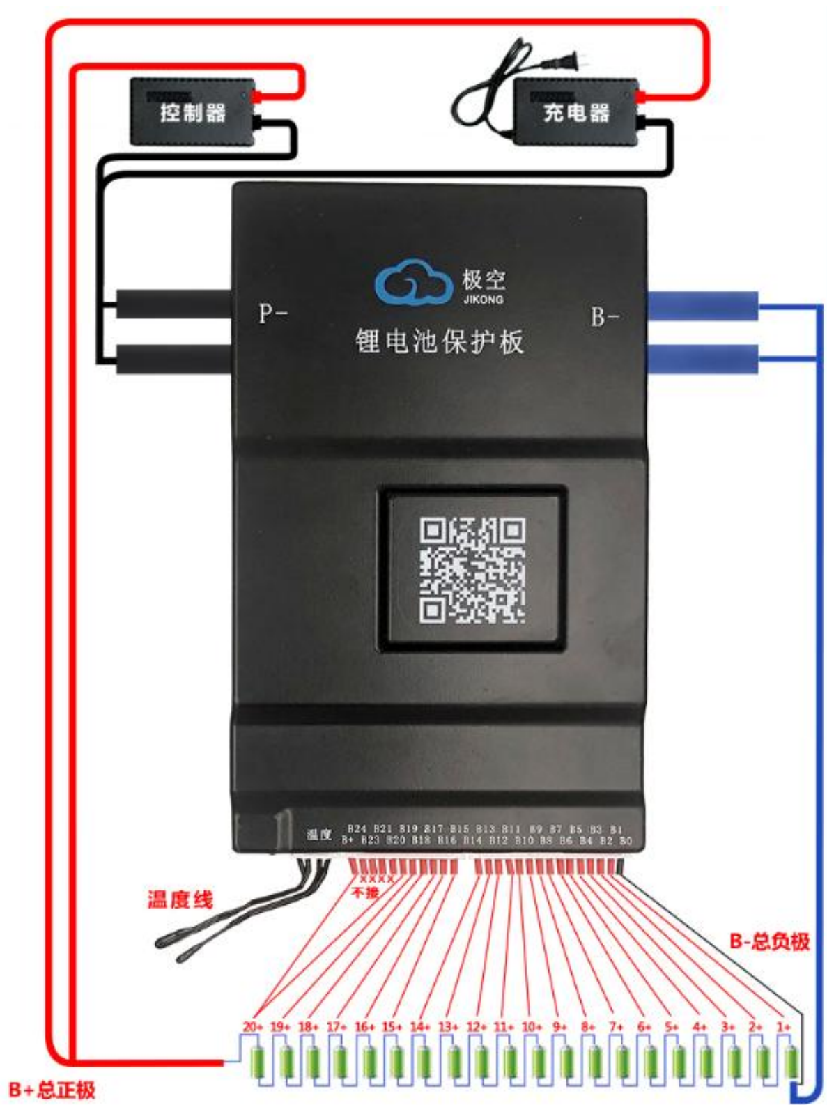
Figure 11. 20S Battery Wiring Diagram
