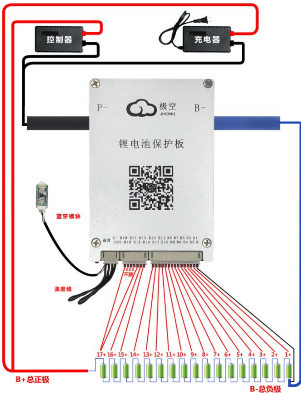
Figure 22. 17S Battery Wiring Diagram
