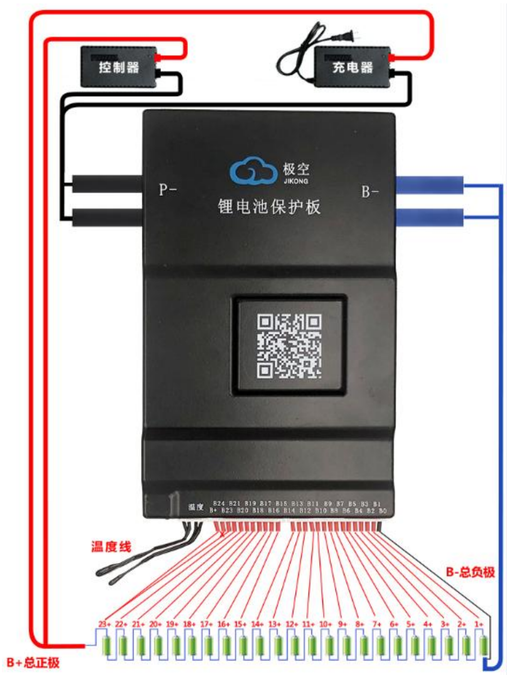
Figure 8. 23S Battery Wiring Diagram
